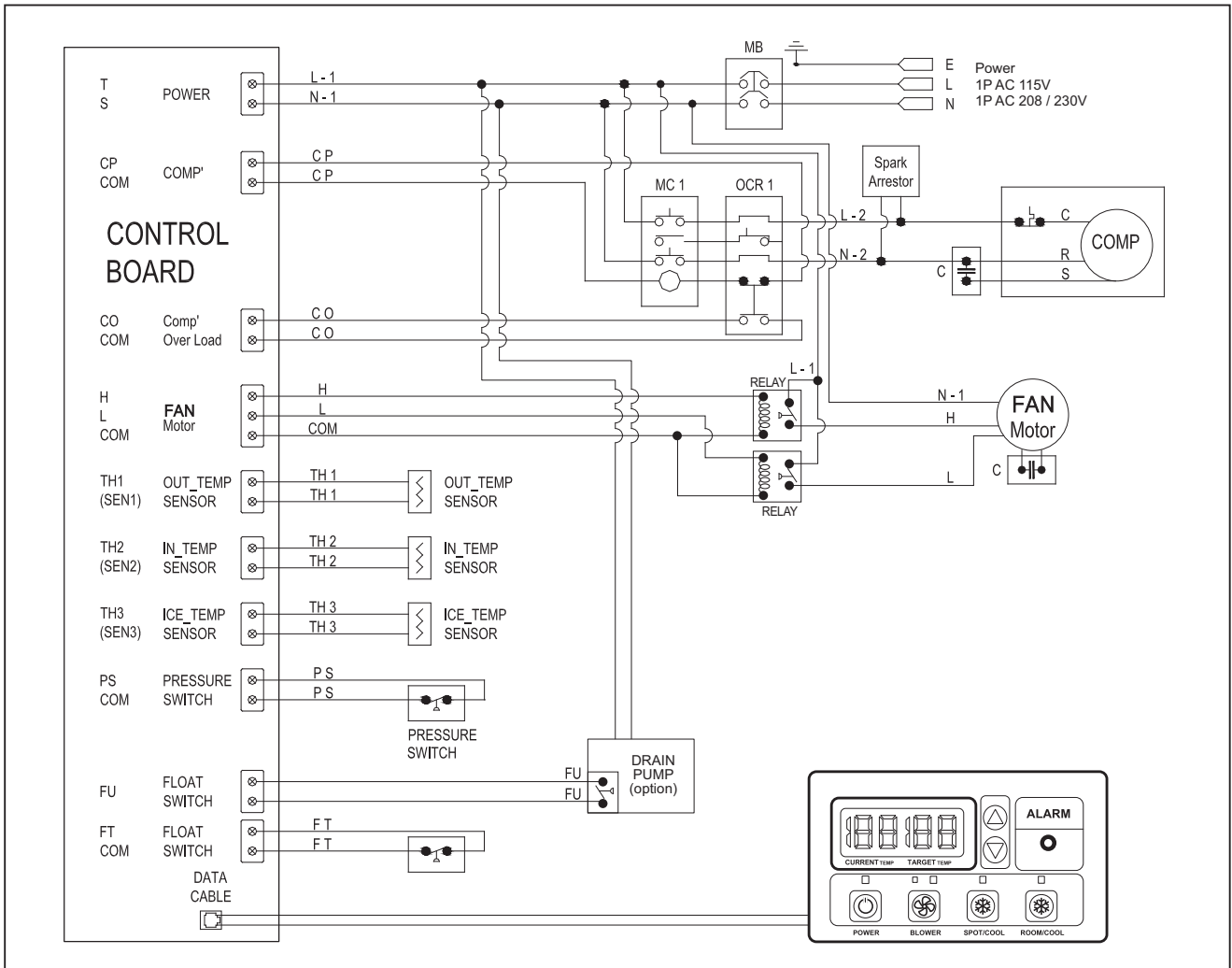
Figure 14 - Circuit Wiring Diagram (WPC-4000)
