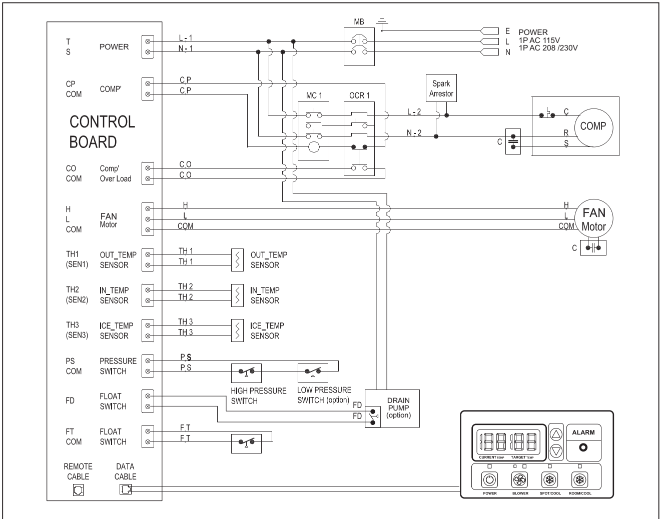
Figure 13 - Circuit Wiring Diagram (WPC-3000,5000)
